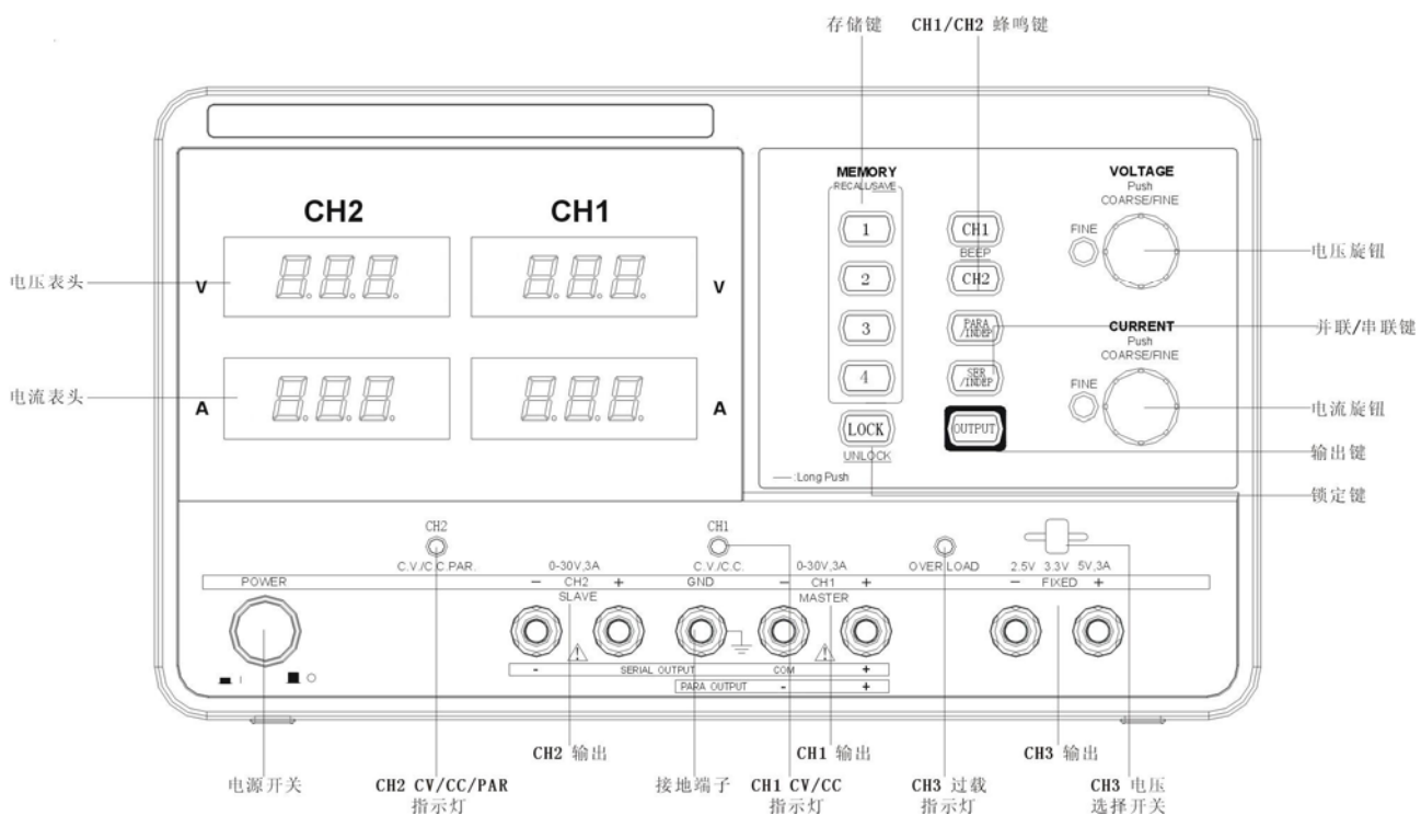
Fig.1.4-2 MPD-3303/3305/3303C/3305C/3303D/3305D 前面板图
