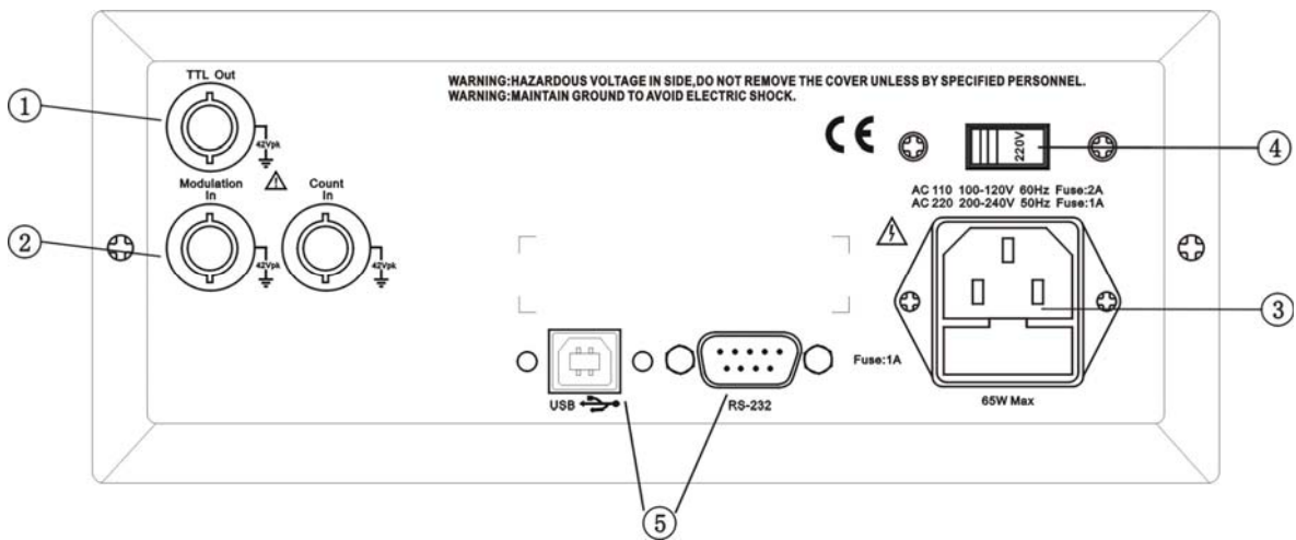
Rear Panel
